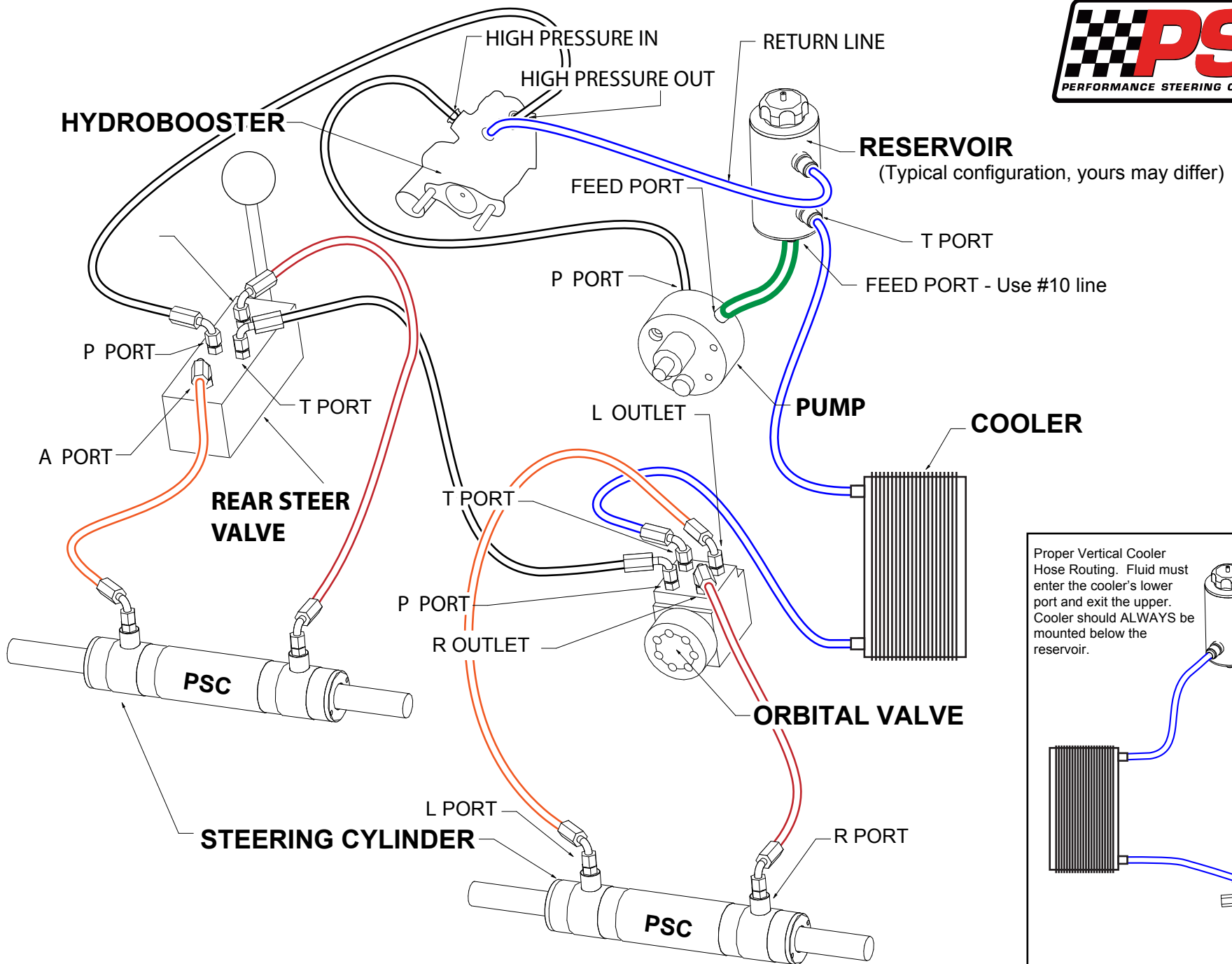
FULL HYDRAULIC HOSE ROUTING FOR FRONT AND REAR STEER APPLICATION WITH HYDROBOOST
