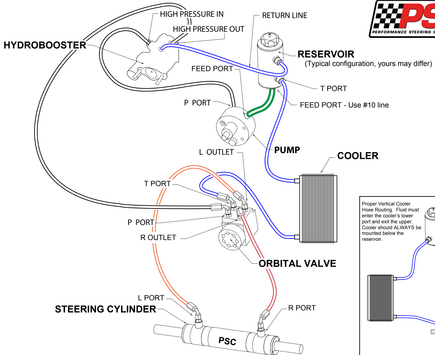
FULL HYDRAULIC HOSE ROUTING FOR FRONT STEER APPLICATION WITH HYDROBOOST
