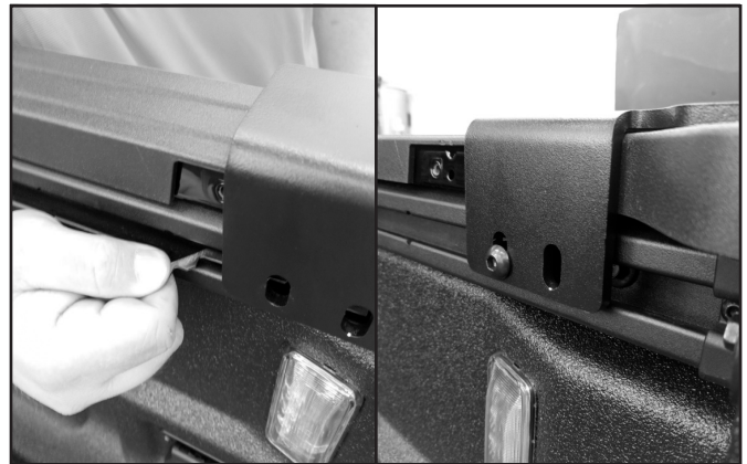
Figure 2 (Left): Using Venture Tec alignment tool to keep pressure on nut plate
