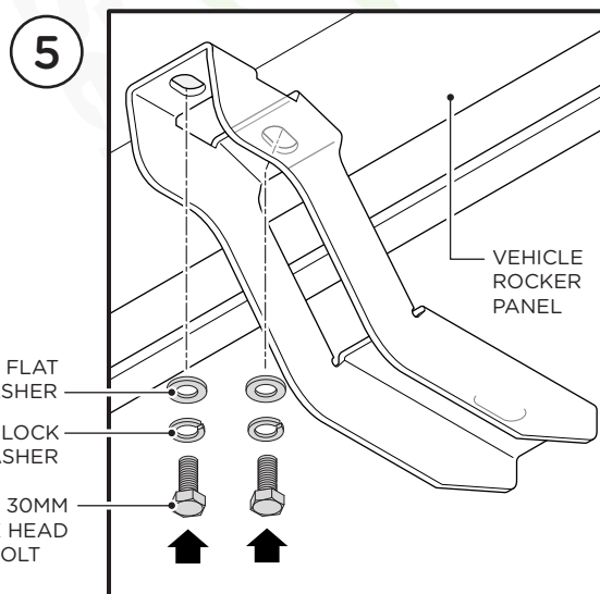
Front Bracket
