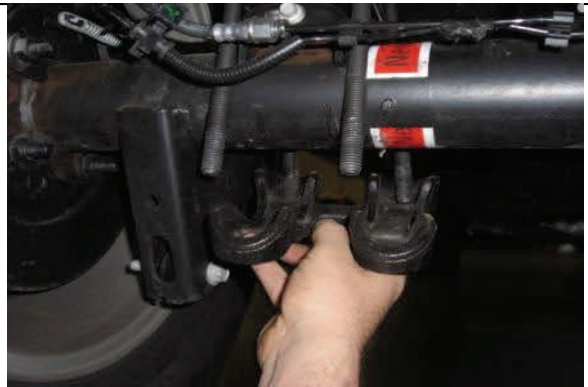
Remove lower u-bolt axle plate.
