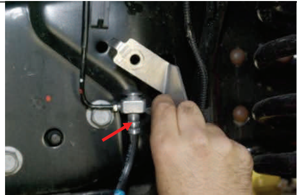
Note line direction, replace OE bracket with new drop bracket
