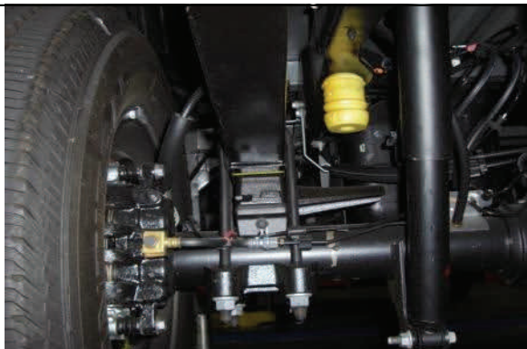
Raise Vehicle and support by frame. Support axle with jack.
