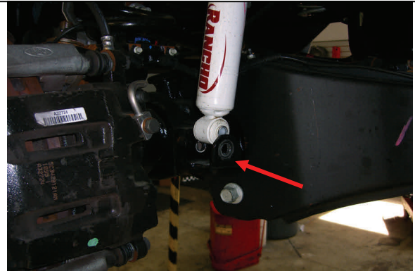
Disconnect dr./pass. front lower shock bolts
