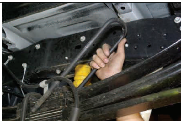
Remove U-bolts and slowly lower axle to remove OE block.
