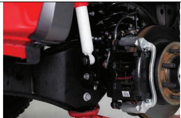
Install and tighten lower shock extension bracket and shock
