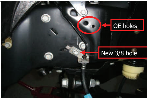
Shown dr. side new 3/8 brake line hole location.
