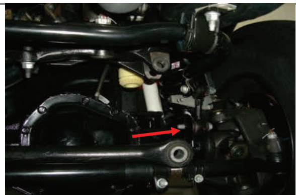
(05-10) disconnect dr/pass lower front sway bar endlink bolt.
