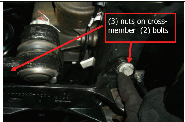
Optional trac bar bracket; Remove mounting hardware (5)
