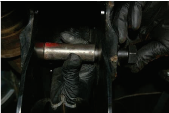
Insert crush sleeves and new hardware into drop bracket.
