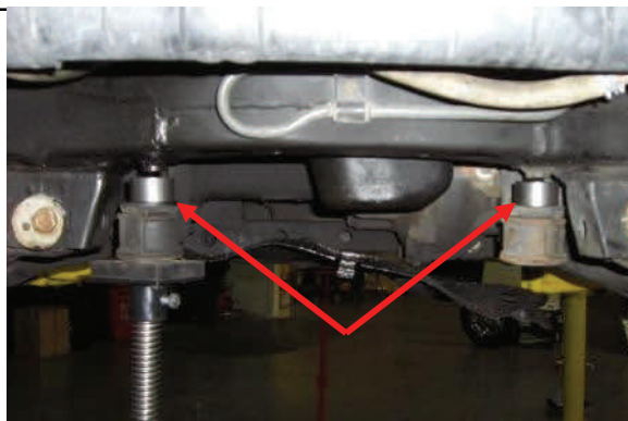
4WD Lower differential and place spacers as shown
