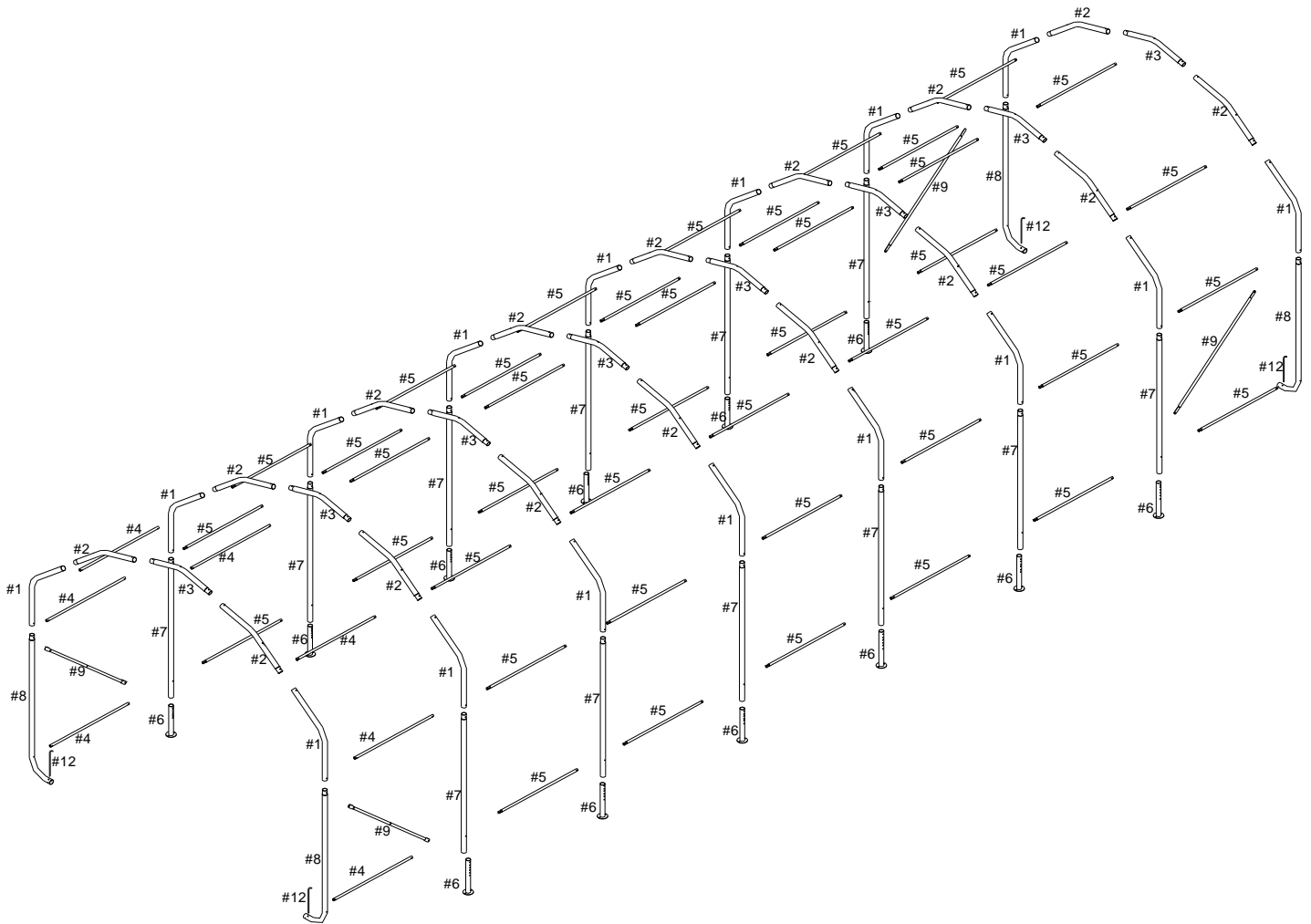
Barn Frame Assembly 12 x 28 x 12
