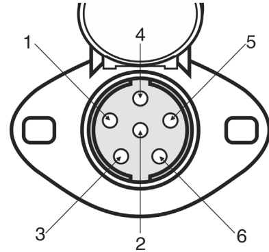
front of 6-wire socket
