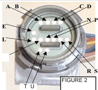
PIN VIEW OF INTERNAL CASE CONNECTOR.
