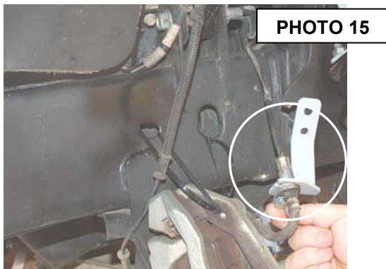
Install the line on the new bracket.
