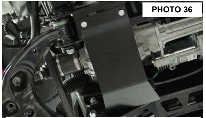
INSTALL THE SKID PLATE
