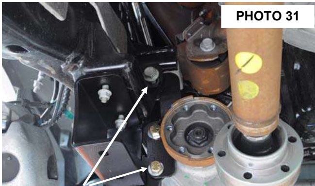
INSTALL THE DR SIDE LOWER REAR DIFF BOLT
