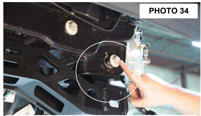
INSTALL THE FRONT CROSS-MEMBER
