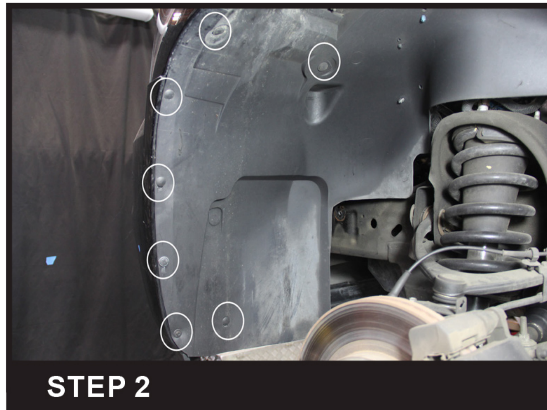
Remove the six clips and the 7mm bolt on the wheel fender liner
