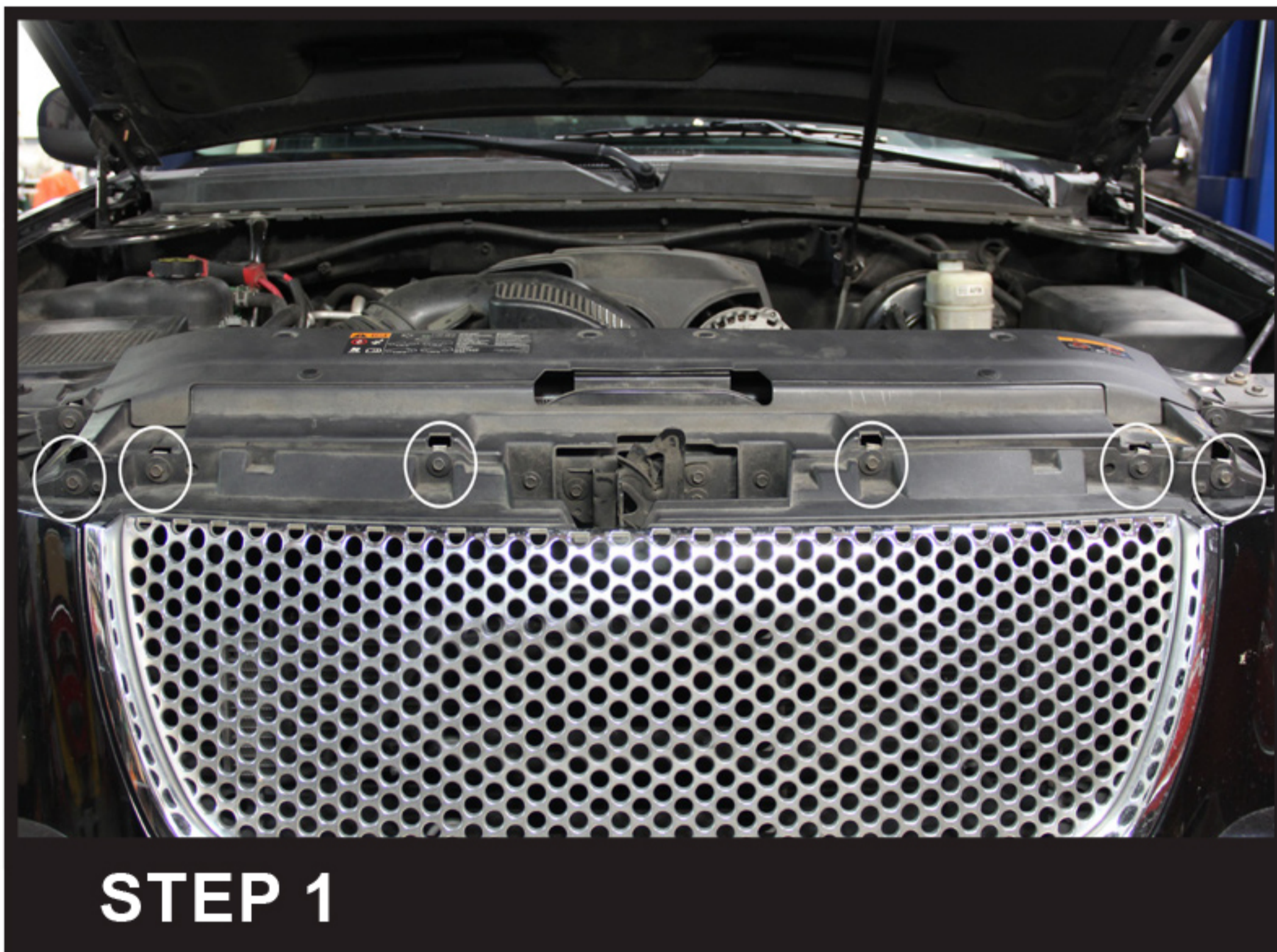
Remove the six 10mm bolts on top of the front grille
