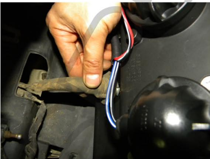
21. Attach the lighting harness to the projector headlight
