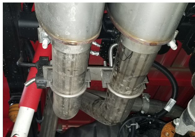
Detail 12: Tail hanger assembly
