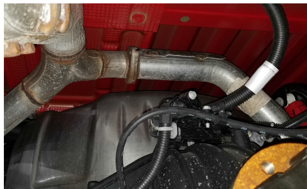
Detail 4: Left tail OEM flange connection
