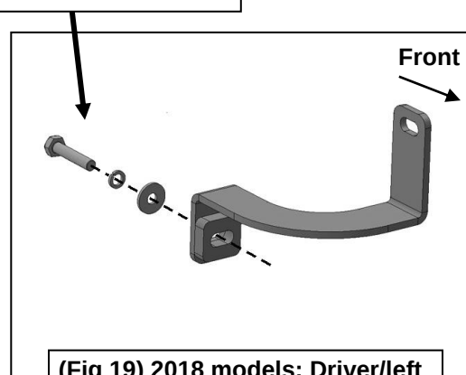
(Fig 19) 2018 models: Driver/left Top Support Bracket
