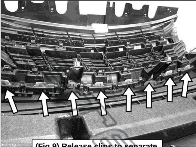
(Fig 9) Release clips to separate grille from bumper (arrows)
