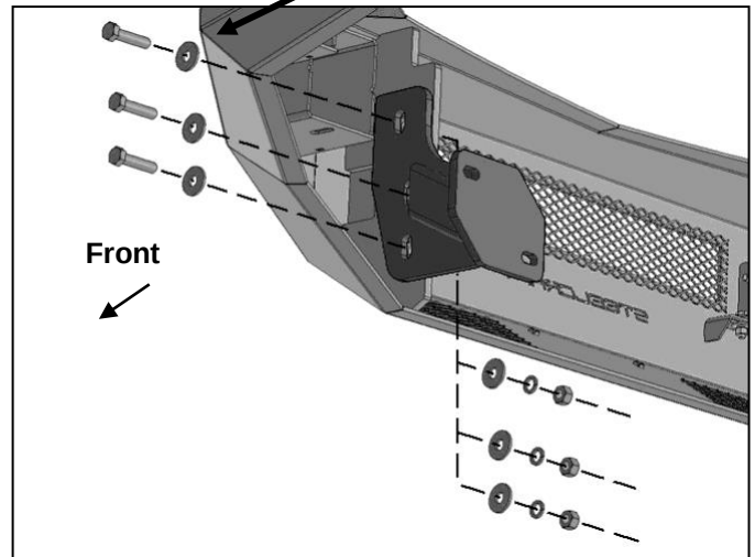
(Fig 18) Attach the Bumper to Frame Bracket
