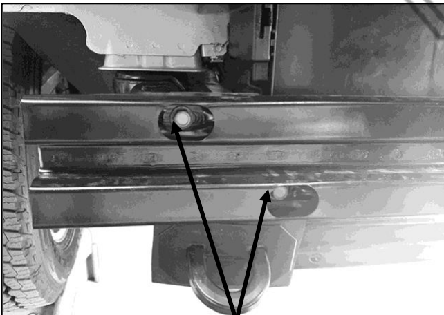
(Fig 11) Remove hex bolts (arrows) to remove impact bumper (passenger side pictured)
