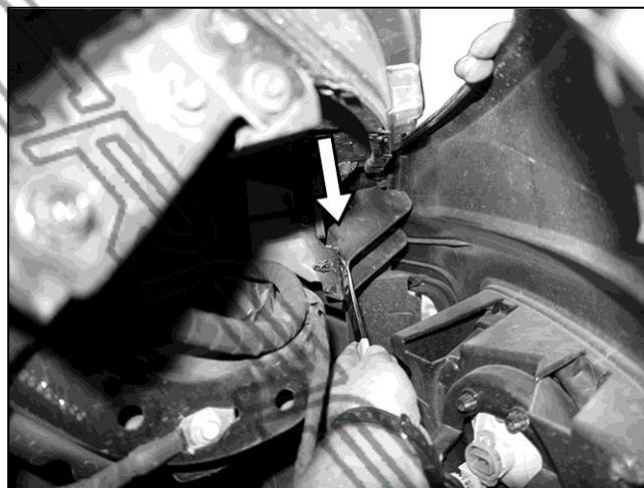
(Fig 8) Pull back loose end of bumper cover to locate inner attachment location for grille below headlight. Use a flat blade screwdriver to carefully pry clips out from bracket to release grille and bumper cover (arrow-passenger/right location pictured)
