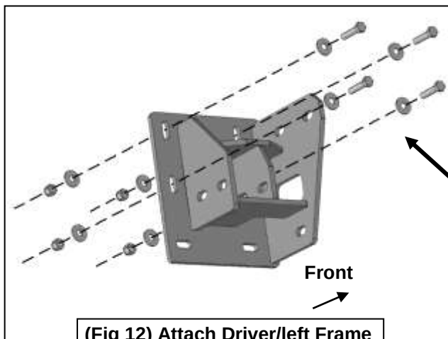
(Fig 12) Attach Driver/left Frame Bracket to end of frame
