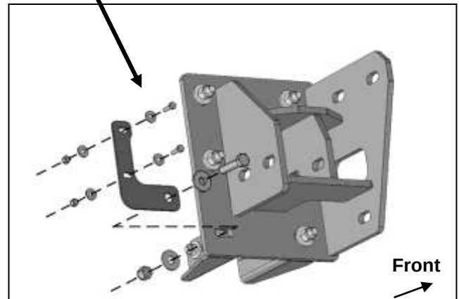
(Fig 19) Attach "L" Relocation Brackets to front of Frame Brackets. Attach shutter assembly, (if equipped), to front of Relocation Brackets
