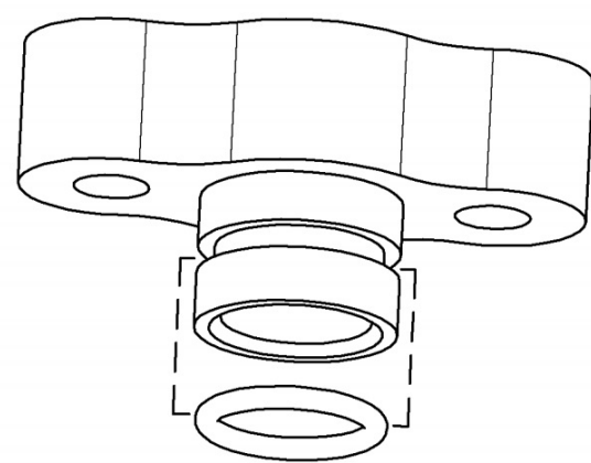
Captive O-Ring
