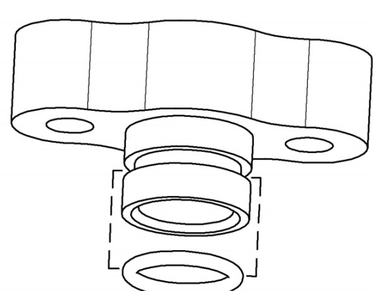
Captive O-Ring
