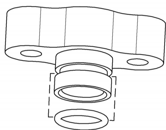
Captive O-Ring
