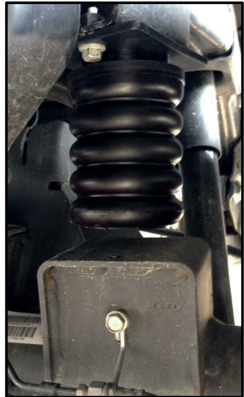
Rear SumoSprings SSR-302-47 installed
