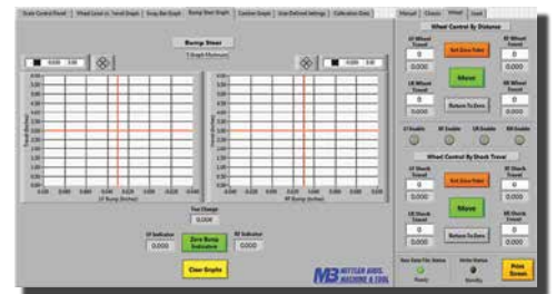
Bump Steer / Camber
