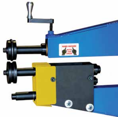
Bead Roller High Throat Adapter Kit see page 23
