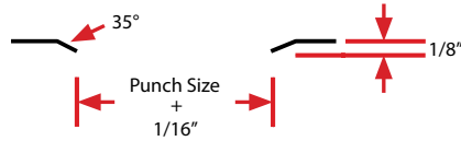
Aircraft Punch / Flare
