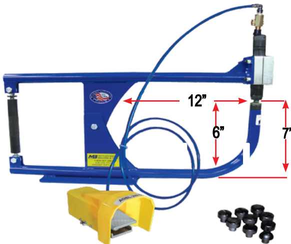
12" Planishing Hammer
