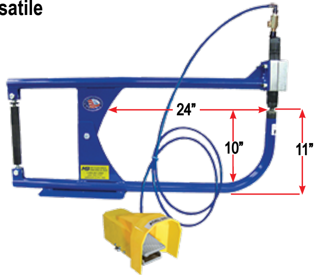
24" Planishing Hammer
