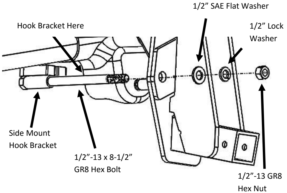
Figure 5.1 (Driver side shown)
