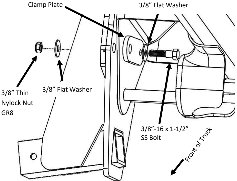
Figure 3.1 (Leaf spring not shown for clarity. Driver side shown)
