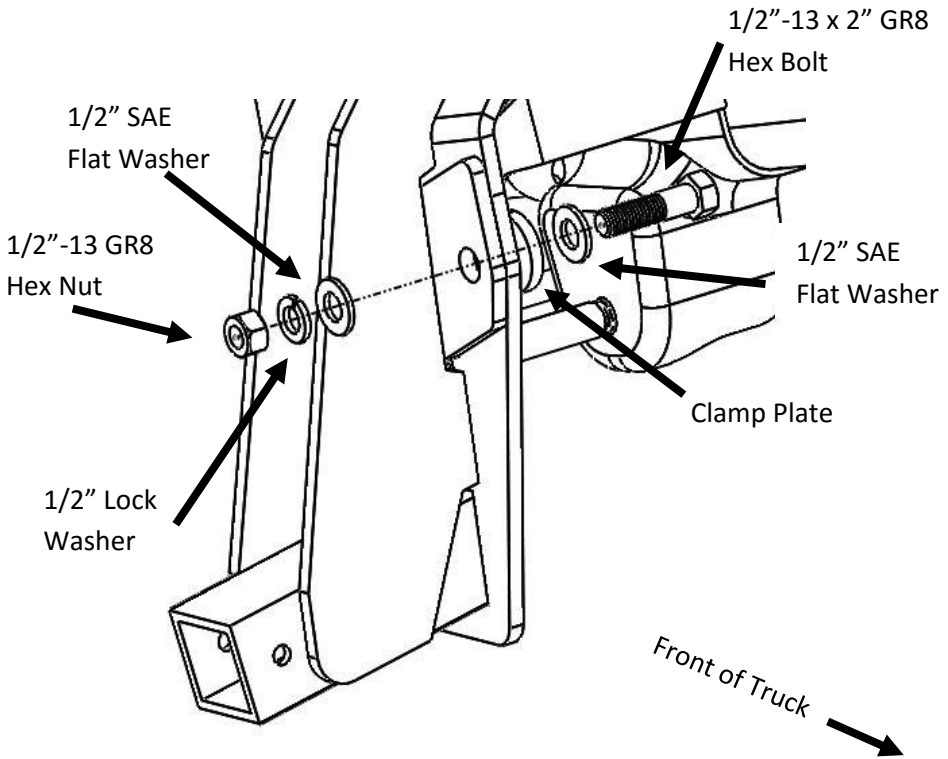
Figure 4.1 (Leaf spring not shown for clarity. Driver side shown)
