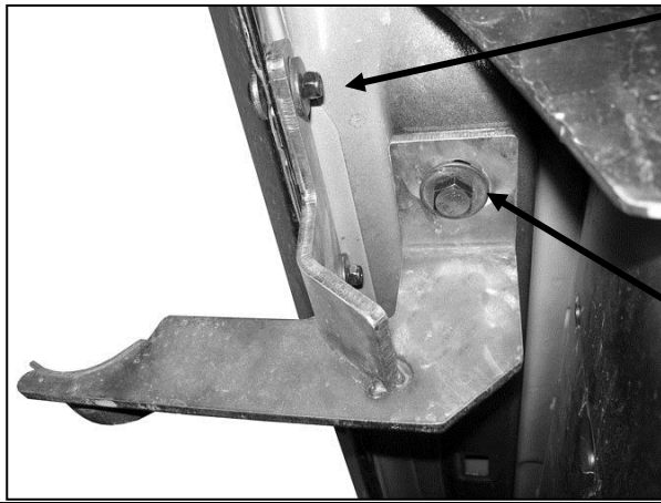
(Fig 3A) Passenger side Front Mounting Bracket installation pictured ("mid length" bracket)
