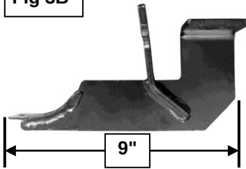
Passenger side "mid-length" front Bracket pictured
