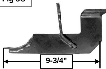
(Fig 3A) Passenger side "long" center Bracket pictured
