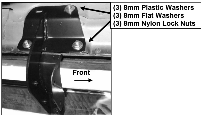
(Fig 4) Driver side front Bracket installation
