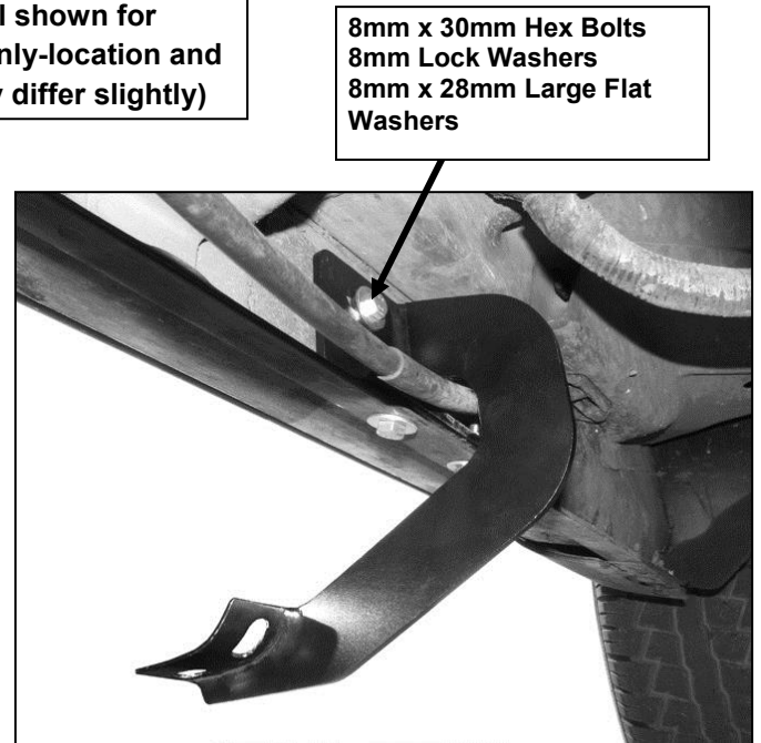
(Fig 2) Driver side-front Mounting Bracket location
