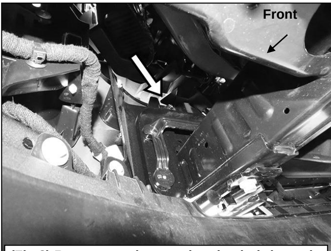
(Fig 8) Remove top bumper bracket bolt (arrow). Driver/left side pictured from below and behind bumper (also see Fig 9)
