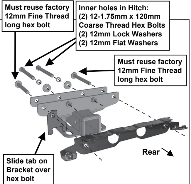
(Fig 4) Receiver Towing Hitch assembly with factory L support bracket and Trailer Harness Bracket
