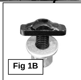
12mm x 35mm T-Bolt Plate 12mm Flat Washer 12mm Lock Washer 12mm Hex Nut
