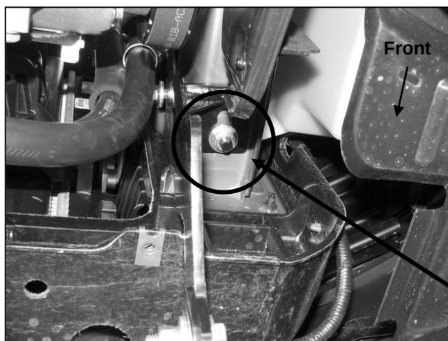
(Fig 7B) Bottom of passenger Frame Bracket attached to Large Bolt Plate pictured from below
