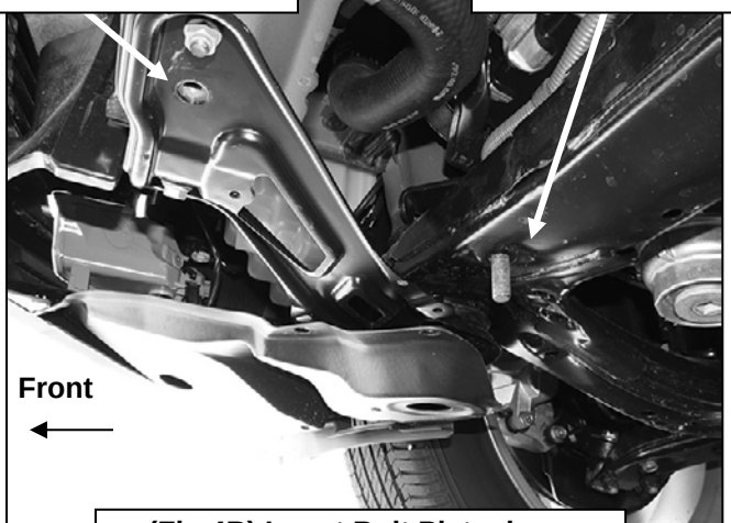
(Fig 4B) Insert Bolt Plate down through holes in cross member
