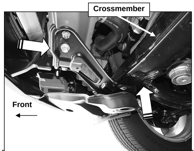
(Fig 2) Passenger side mounting location (arrows)
