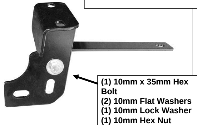
(Fig 3) Driver side Support Bracket in "no Tow Hook" position
