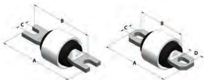
"BP" BAR PIN MOUNTING DIMENSIONS EB1 WITH BUSHING AND BAR PIN
