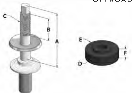
"S" Stem Bushing Mounting Dimensions
