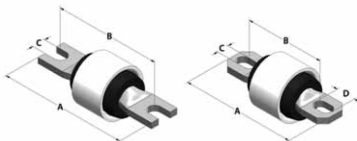
"BP" Bar Pin Mounting Dimensions
