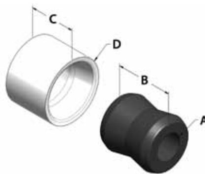
"EB" Eyelet Bushing Mounting Dimensions
